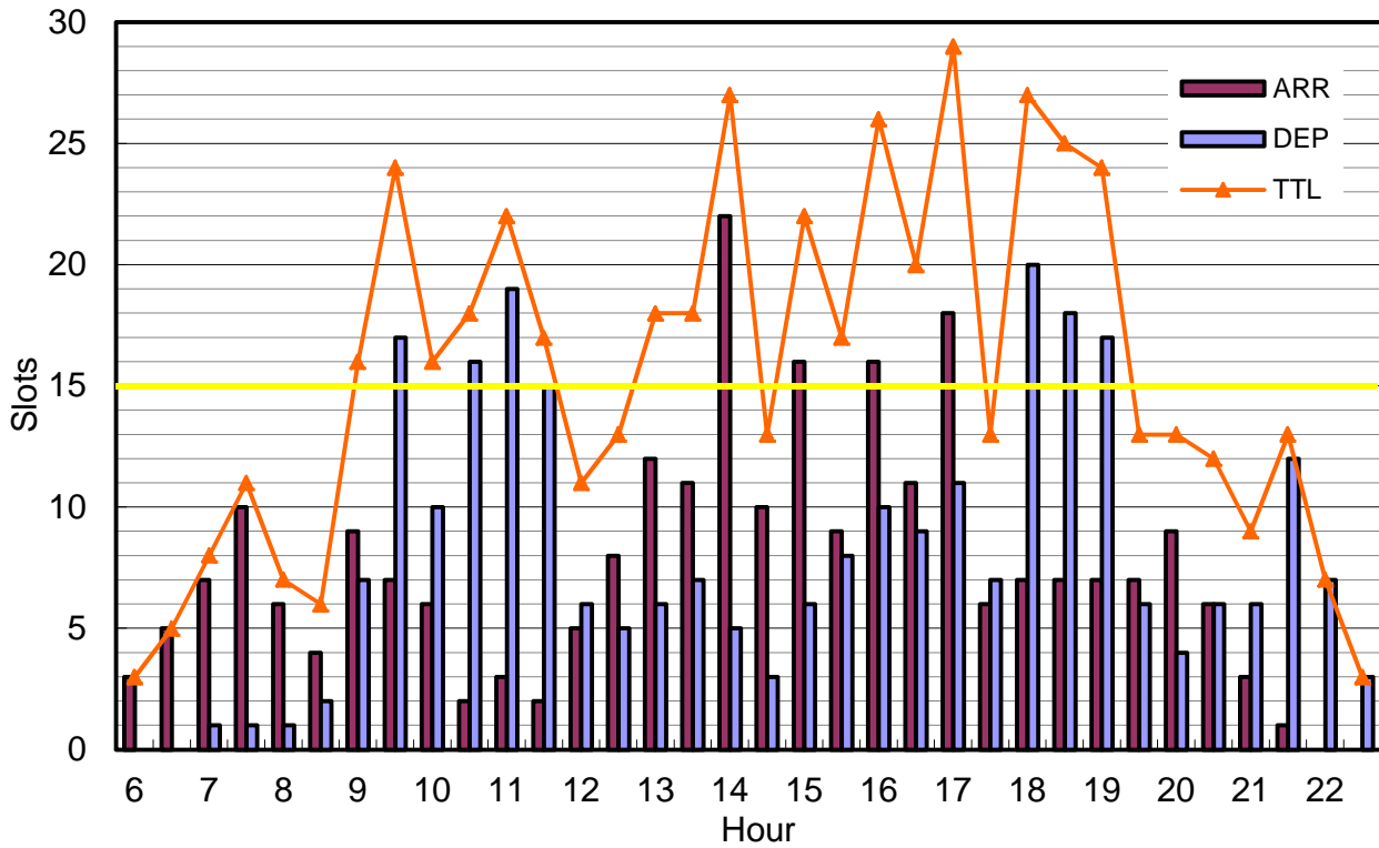
Peak Demand
