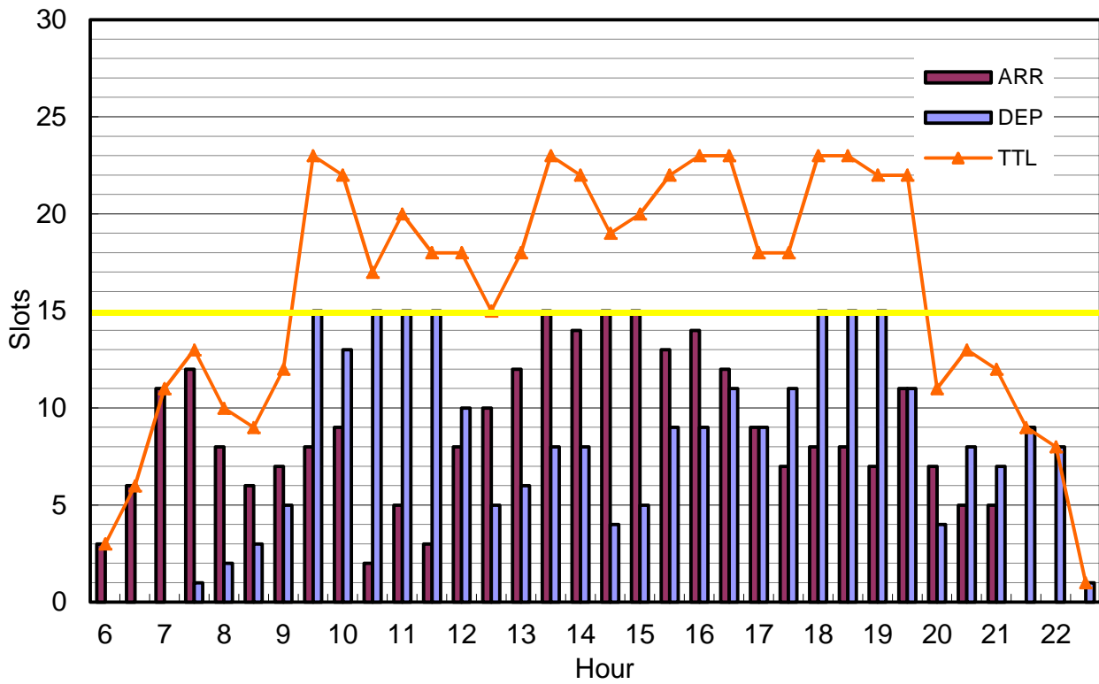
After Coordination
